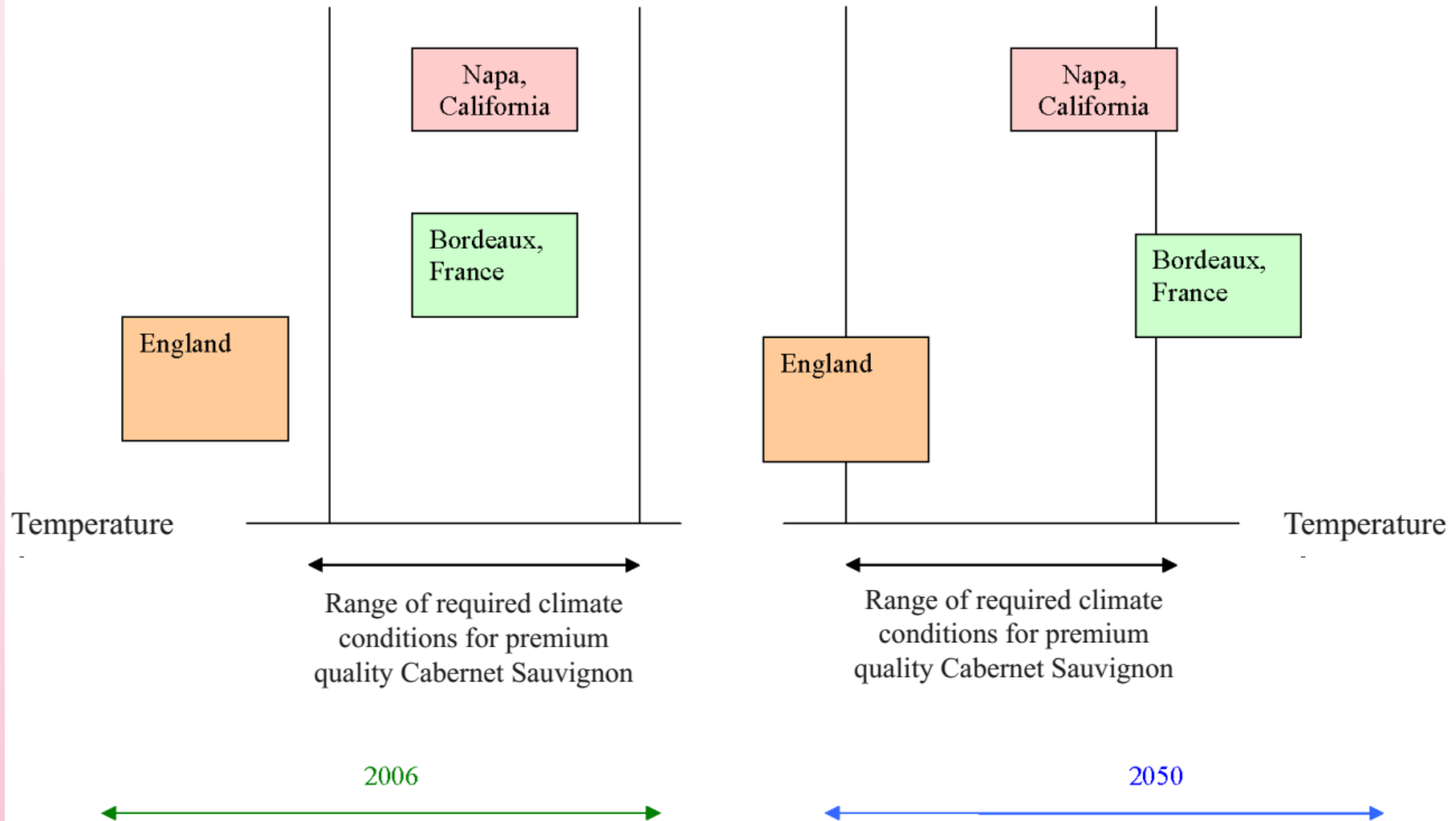
Figure 7: Illustration of Current Average Temperatures in Several Regions and Required Climate Conditions for Premium Quality Cabernet Sauvignon
